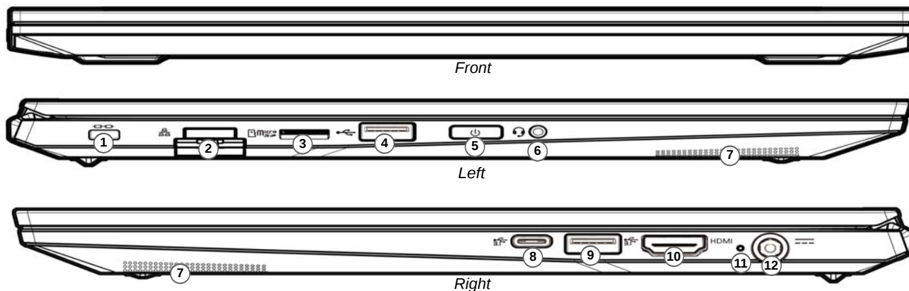
Figure 9 - Front, Left & Right Views (Model A)
