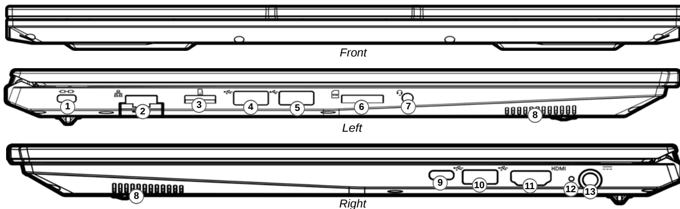
Figure 11 - Front, Left & Right Views (Model C)
