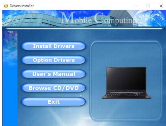
Figure 19 - Install Drivers
