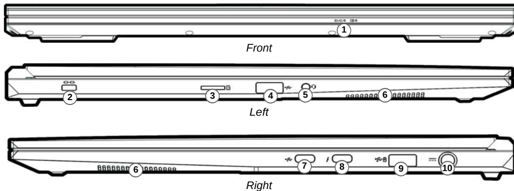
Figure 8 - Front, Left & Right Views (Model B)
